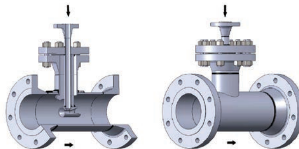
VENTURI DESUPERHEATERS ATEMPERATOR
