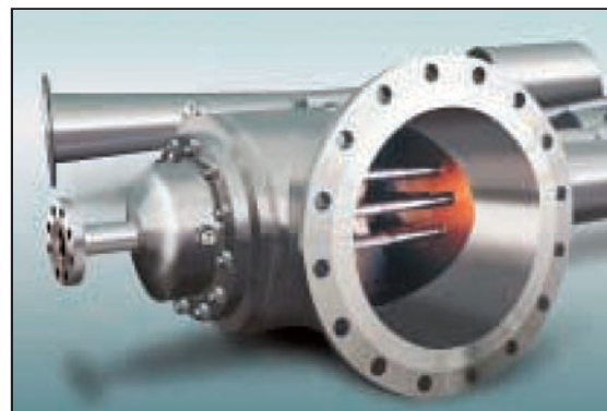
Multiple-Nozzle assembly viewed through the suction connection.
